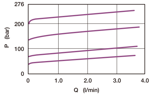
► Pressure Differential vs. Flow (Range A)
