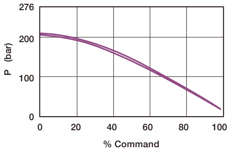
► Pressure vs. Command (Range A)
